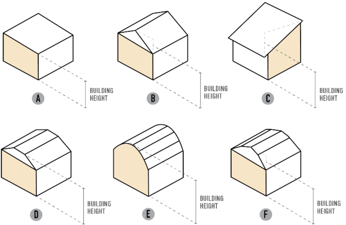
Figure 2-1: Interpretation of Building Height Measurement
