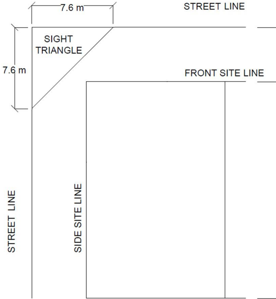
Figure 2-3: Sight Triangle
