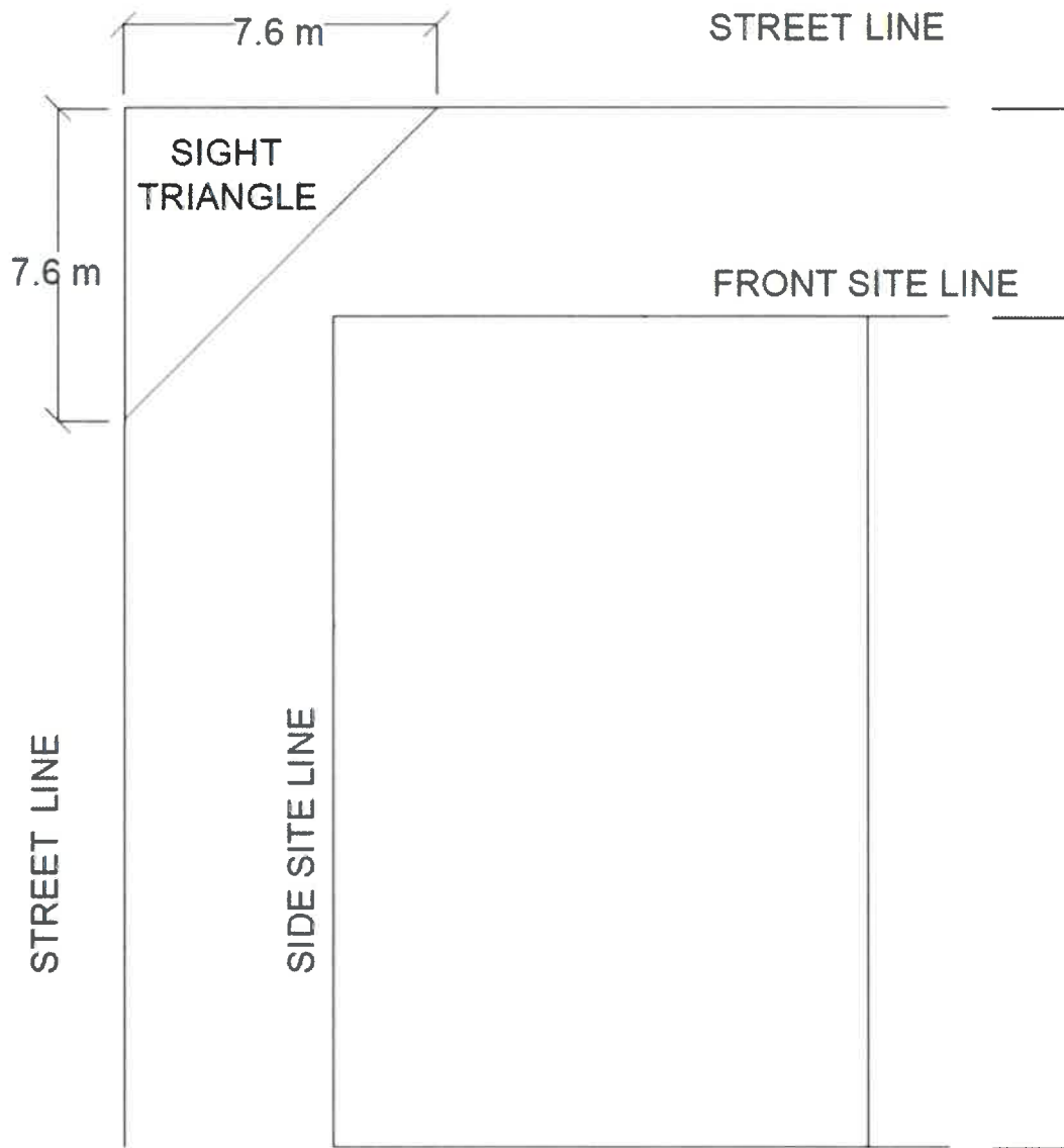
Figure 2-3: Sight Triangle
