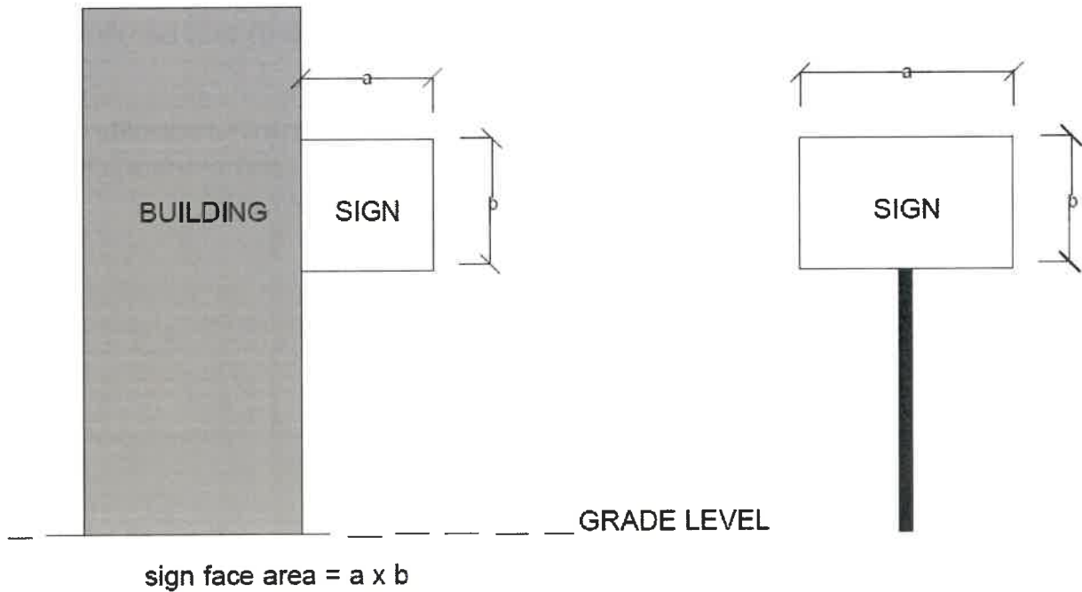
Figure 2-2: Calculation of Sign Face Area
