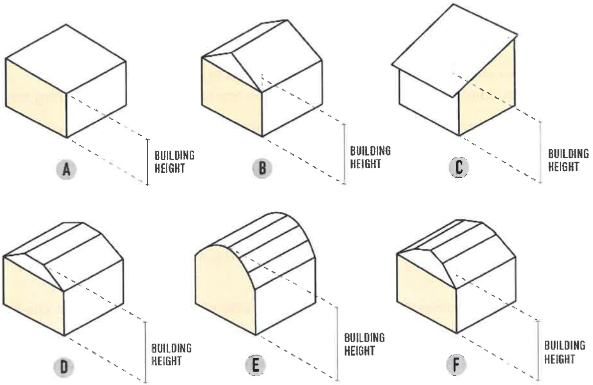
Figure 2-1: Interpretation of Building Height Measurement
