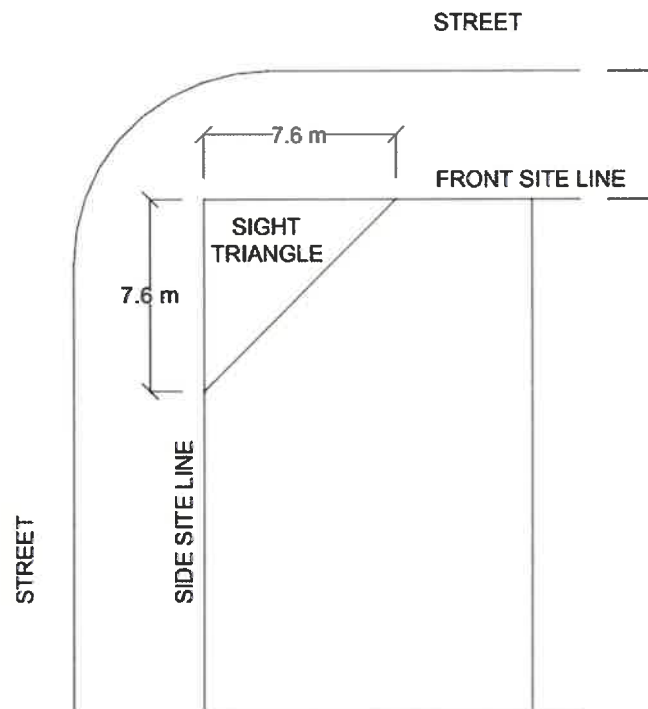
FIGURE 2-3: Sight Triangle
