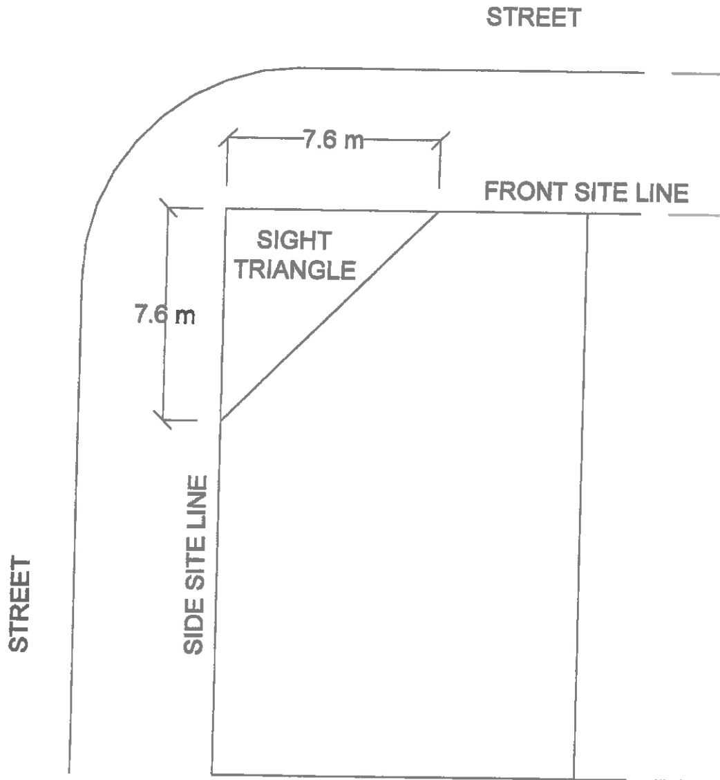
FIGURE 2-3: Sight Triangle
